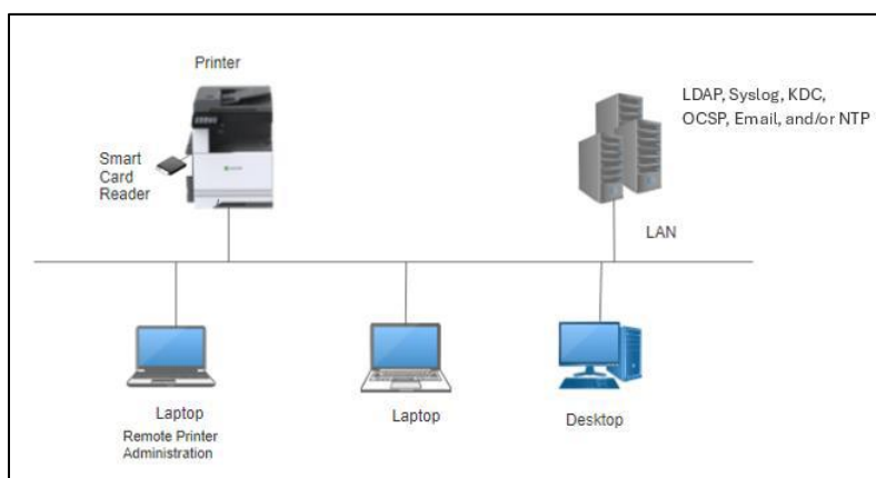
Figure 1: TOE Architecture
